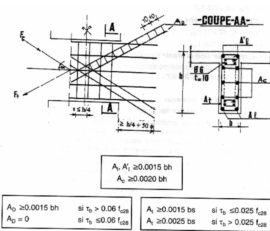
Figure 7.11 Armatures de linteaux
